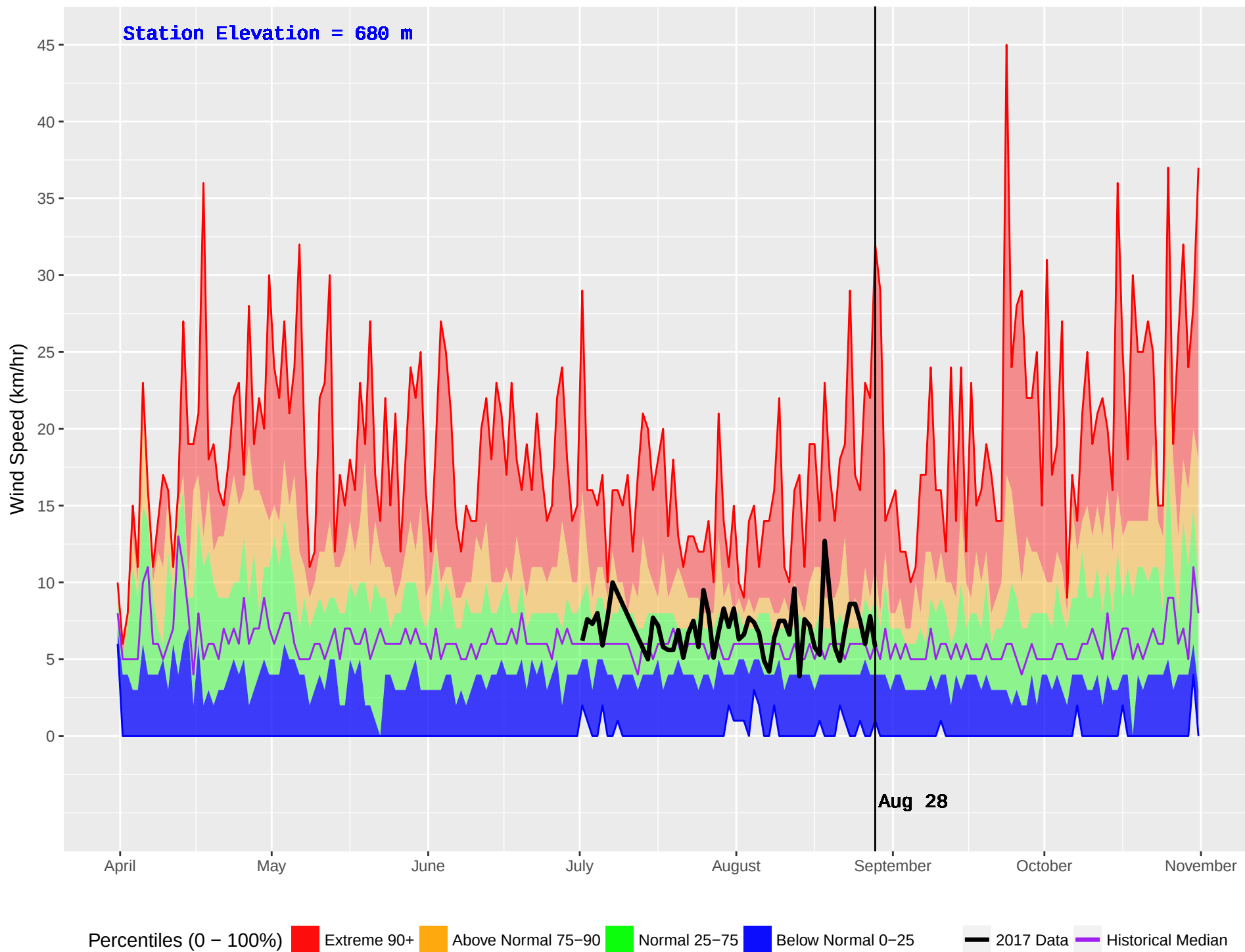
SUMMIT (11) : Historical (1985–2016) and Current (2017) Noon Wind Speed
